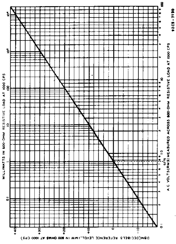
Figure 9. Graph for conversion of rms voltages to dbm values
