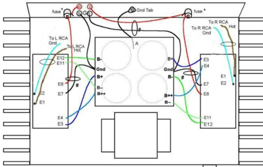
XL-280 BASIC LAYOUT
