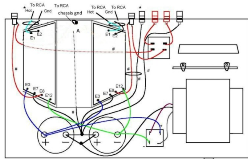
DH-500 BASIC LAYOUT
