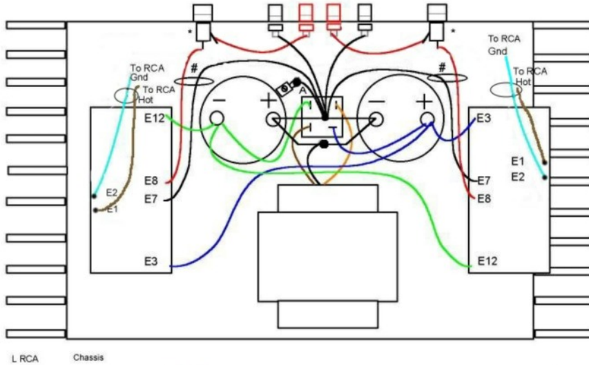
PA-5 Fig. B DH-200/220 BASIC LAYOUT
